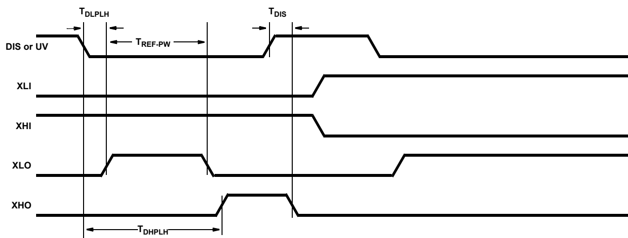
FIGURE 3. DISABLE FUNCTION
