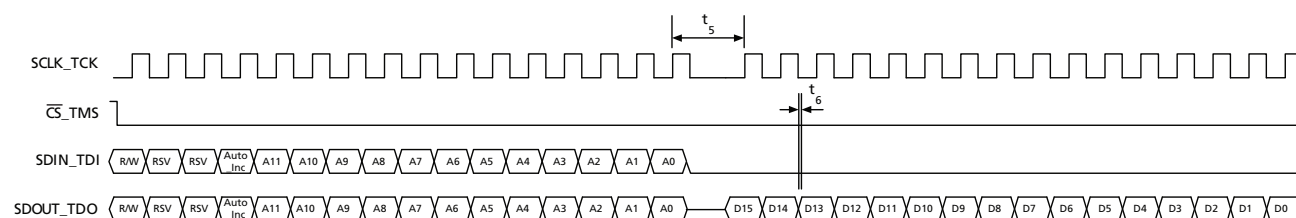
Figure 4-25: Read Mode
