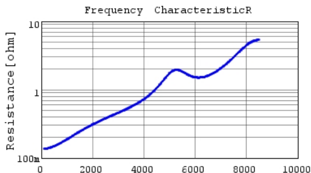
GRM1555C1H130JA01 R DCOV,25degC
