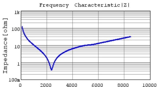
GRM1555C1H130JA01 |Z| DCOV,25degC
