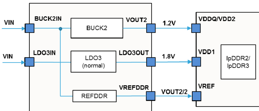
Figure 40. Powering lpDDR2/lpDDR3 memory (LDO3 normal mode supplied from VIN)
