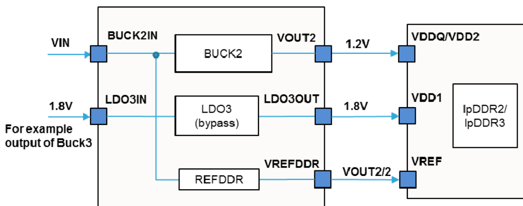
Figure 39. Powering lpDDR2/lpDDR3 memory (LDO3 in bypass mode)
