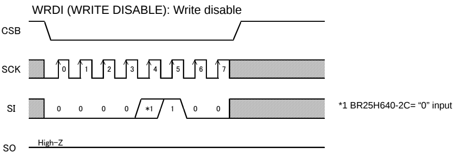
Figure 36. Write disable
