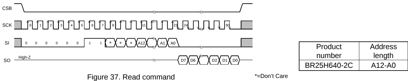
Figure 37. Read command
