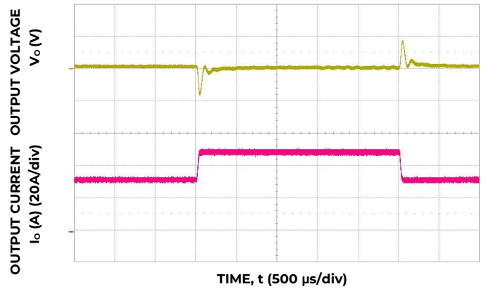
Figure 4. Typical Transient Response to 1.0A/ \mu s Step Change in Load from 50% to 75% to 50% of Full Load, C_o = 470\mu F and 50 V dc Input.
