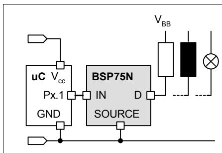
Figure 8 Application Circuit
