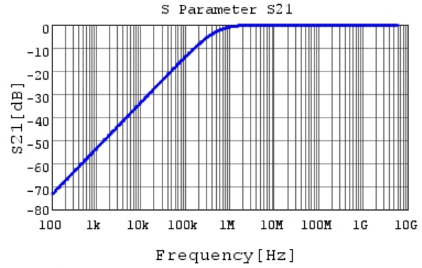
GCM155R71H332KA37 S21 DC0V, 25degC
