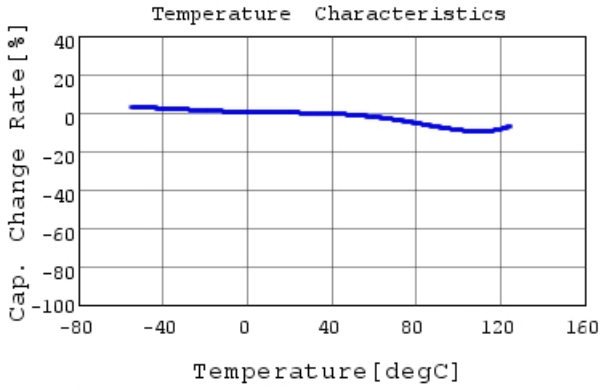
GCM155R71H332KA37 C-Temp. capchange, DC0.0V,
