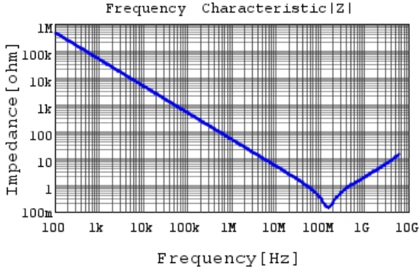
GCM155R71H332KA37 |Z| DCOV, 25degC
