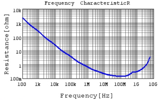
GCM155R71H332KA37 R DCOV, 25degC
