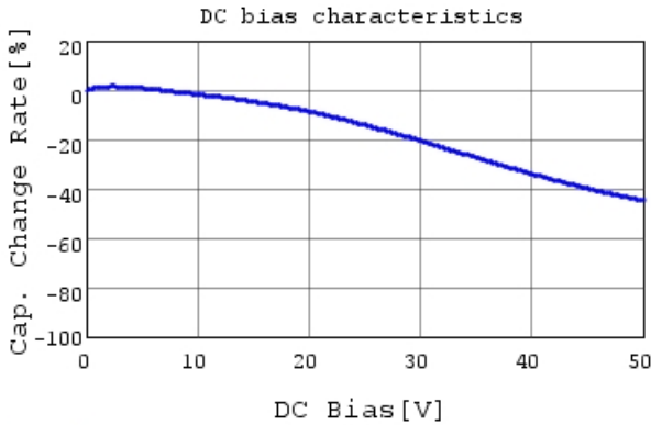
GCM155R71H332KA37 C-DC bias capchange, 25.0c
