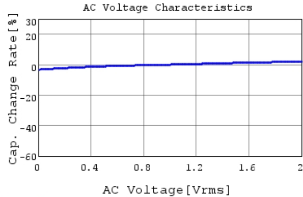
GCM155R71H332KA37 C-AC Voltage capchange, Dc
