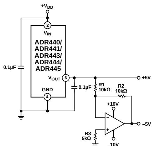
Figure 38. ADR440/ADR441/ADR443/ADR444/ADR445 Bipolar Outputs
