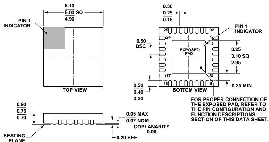
COMPLIANT TO JEDEC STANDARDS MO-220-WHHD. Figure 34. 32-Lead Lead Frame Chip Scale Package [LFCSP] 5 mm x 5 mm Body and 0.75 mm Package Height (CP-32-7) Dimensions shown in millimeters
