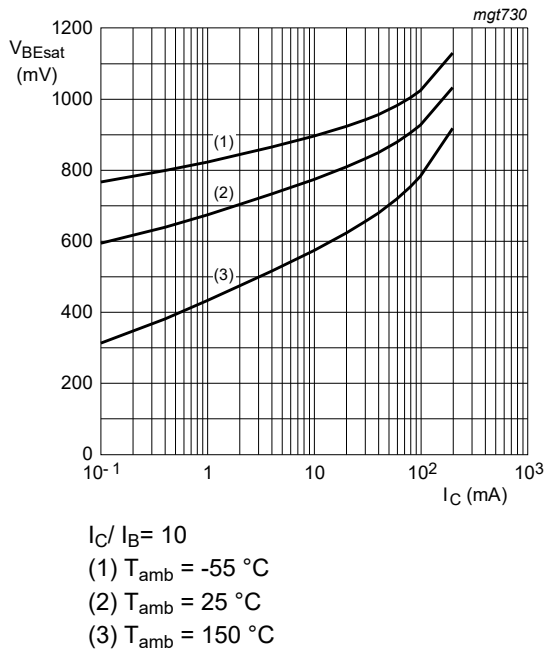
Fig. 11. BC847BQB: Base-emitter saturation voltage as a function of collector current; typical values
