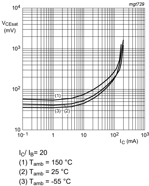
Fig. 10. BC847BQB: Collector-emitter saturation voltage as a function of collector current; typical values
