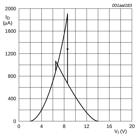
Fig 8. Typical drain current as a function of input
