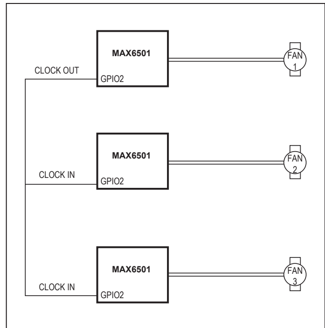
Figure 14. Synchronizing Fans
