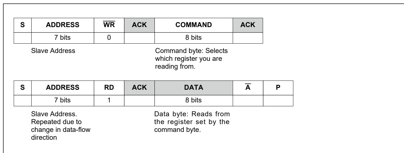
Figure 2b. SMBus Protocol: Read Byte Format
