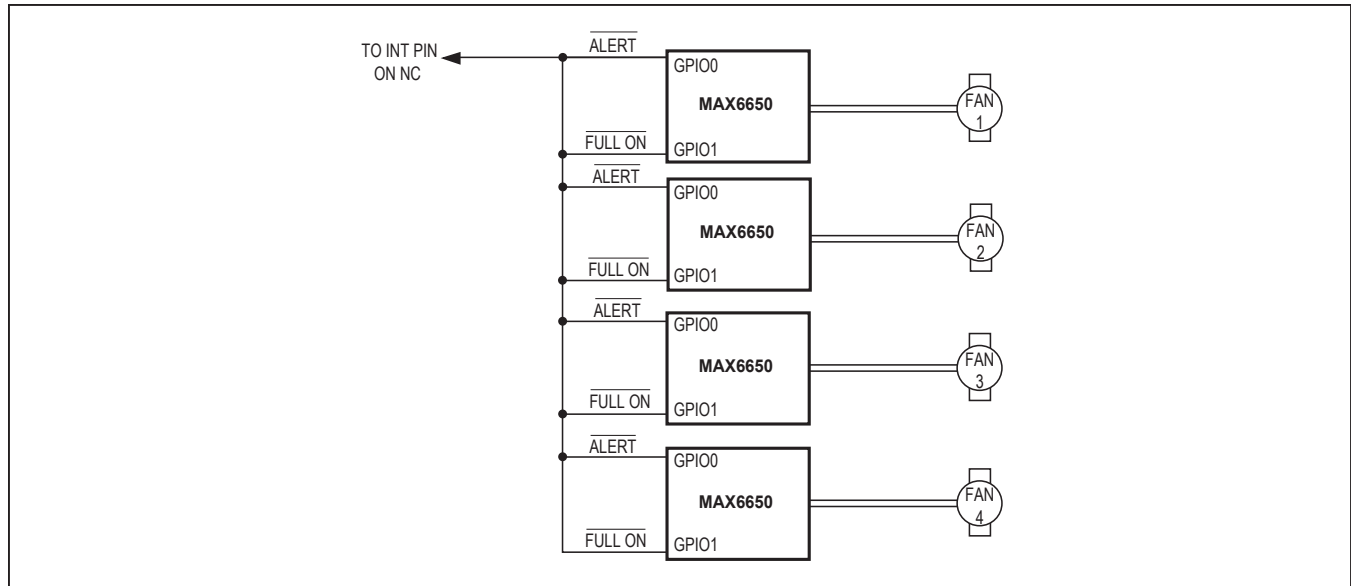
Figure 9. N + 1 Application
