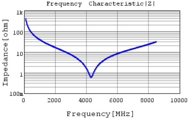
GRM1555C1H3R9WA01 |Z| DCOV, 25degC
