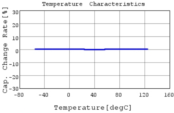
GRM1555C1H3R9WA01 C-Temp. capchange, DCOV, 1
