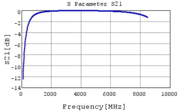
GRM1555C1H3R9WA01 S21 DCOV, 25degC
