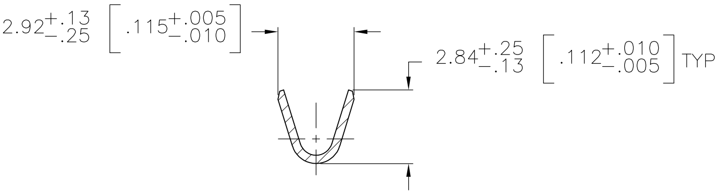
SECTION B-B
