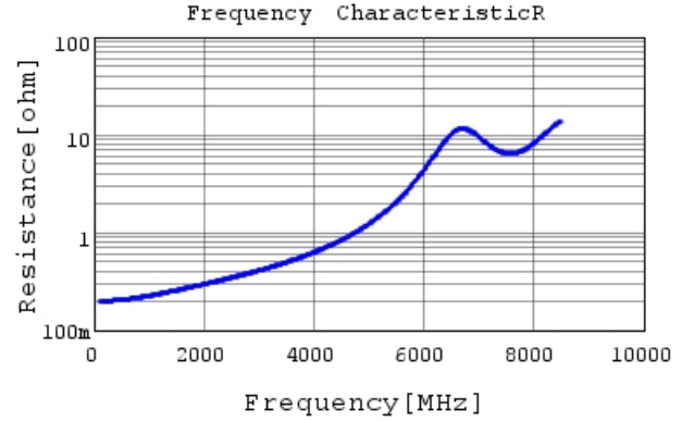
GRM1555C1H7R5BA01 R DC0V, 25degC
