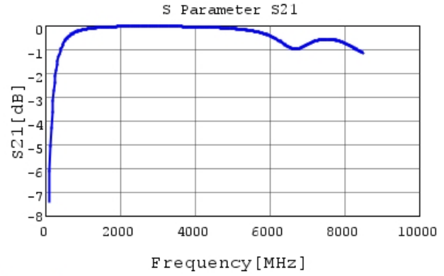
GRM1555C1H7R5BA01 S21 DCOV, 25degC
