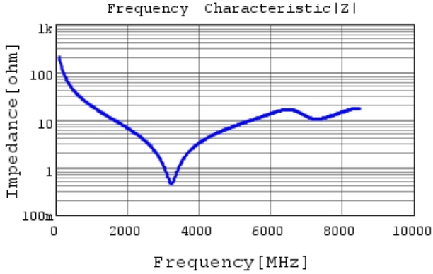
GRM1555C1H7R5BA01 |Z| DC0V, 25degC
