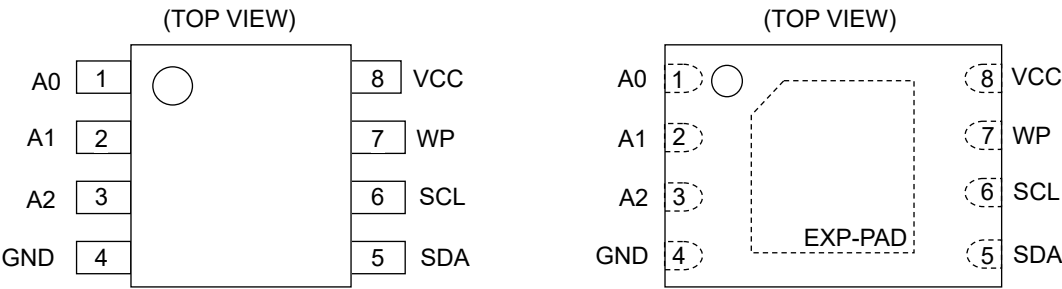
Figure 3-(a). Pin Configuration (SOP8 *1 , SOP-J8, TSSOP-B8, MSOP8) *1 Not Recommended for New Designs.
