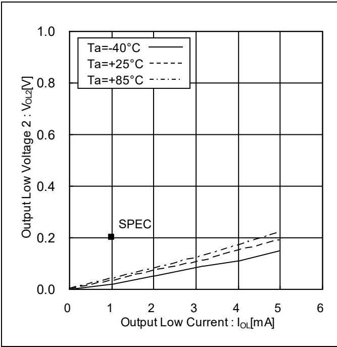
Figure 9. Output Low Voltage 2 vs Output Low Current ( V_{CC}=1.6\text{V} )
