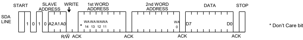
Figure 41. Byte Write
