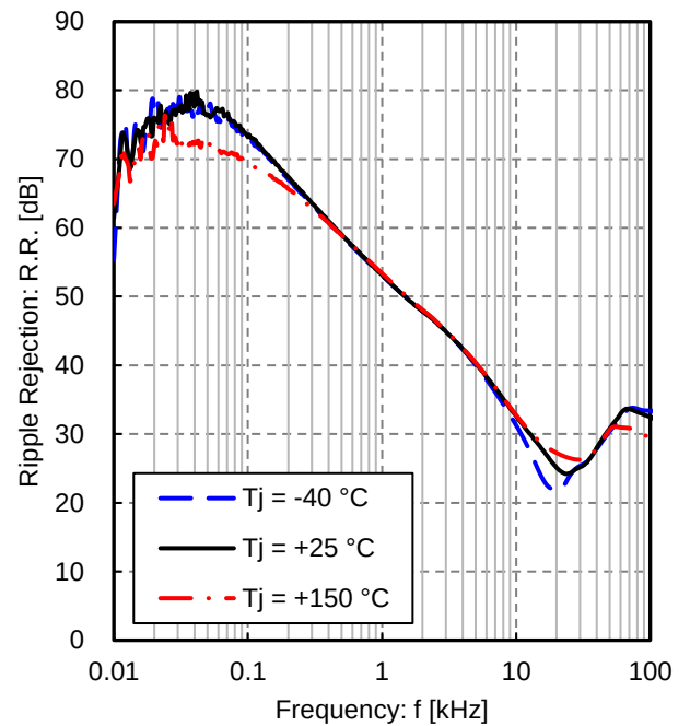
Figure 14. Ripple Rejection (V ripple = 1 V rms , I OUT = 100 mA)
