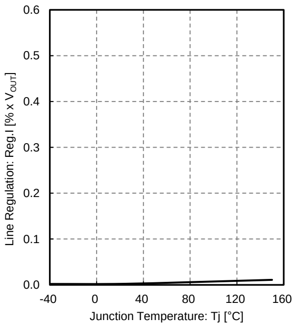
Figure 15. Line Regulation (V IN = 6 V → 28 V)
