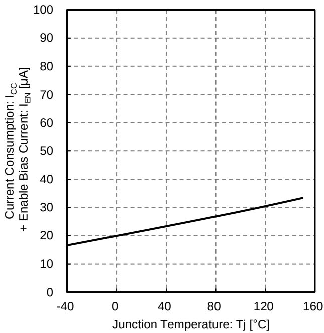
Figure 5. Current Consumption + Enable Bias Current vs Junction Temperature
