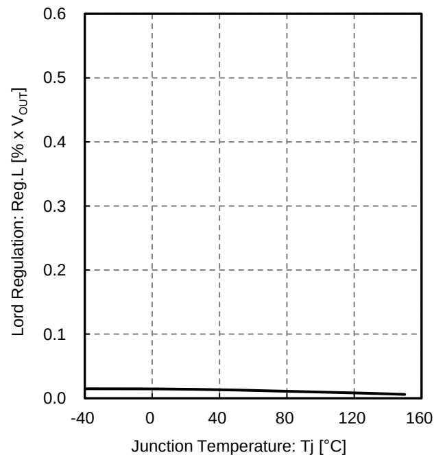
Figure 16. Load Regulation (I OUT = 0.5 mA → 400 mA)
