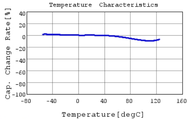
GCM155R72A471KA37 C-Temp. capchange, DC0.0V,
