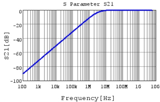
GCM155R72A471KA37 S21 DC0V,25degC
