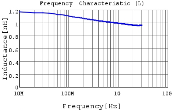
LQP02TN1N0B02 L
