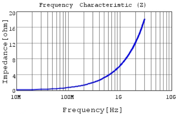
LQP02TN1N0B02 |Z|
