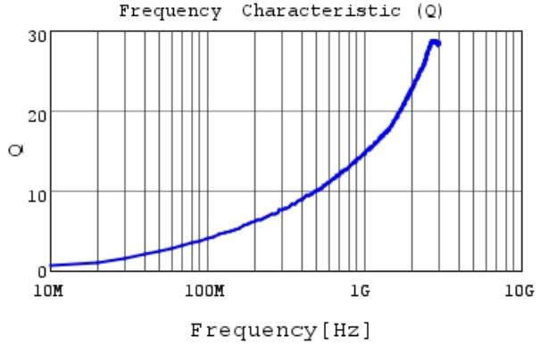
LQP02TN1N0B02 Q
