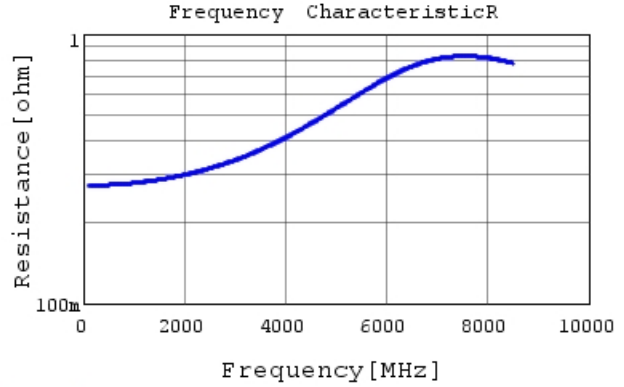
GCM1555C1H3R0CA16 R DC0V, 25degC
