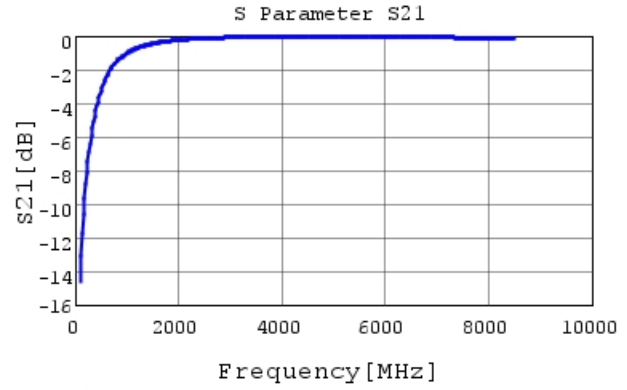
GCM1555C1H3R0CA16 S21 DCOV, 25degC
