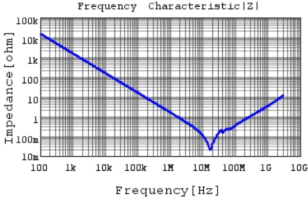
GRJ43DR72J104KWJ1 |Z| DCOV, 25degC
