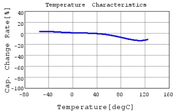
GRJ43DR72J104KWJ1 C-Temp. capchange, DCOV, 1
