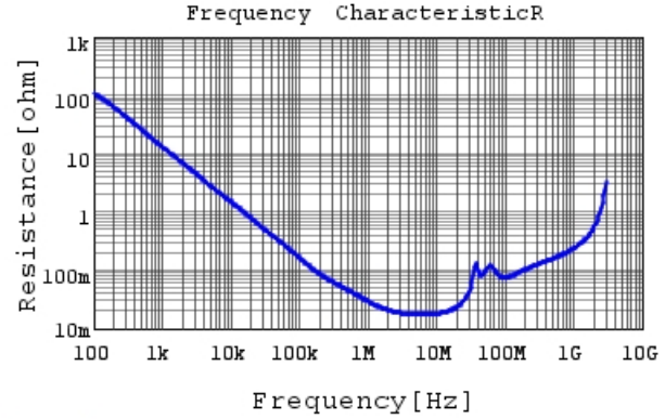
GRJ43DR72J104KWJ1 R DCOV, 25degC
