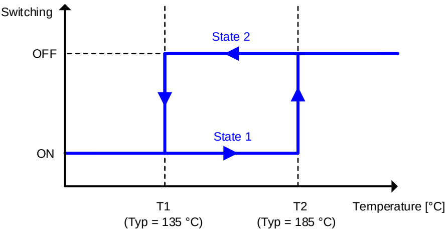
Figure 14. Thermal Shutdown Function
