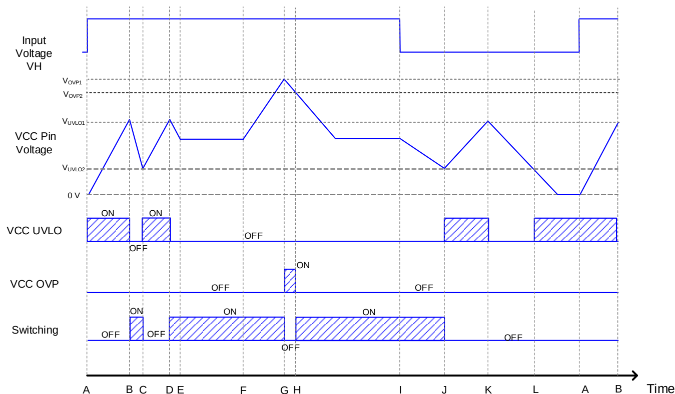
Figure 2. VCC UVLO/OVP (Auto Restart Mode)
