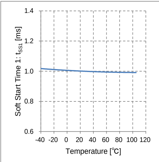
Figure 39. Soft Start Time 1 vs Temperature
