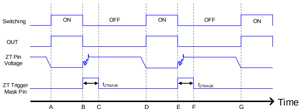
Figure 9. ZT Pin Trigger Mask Function
