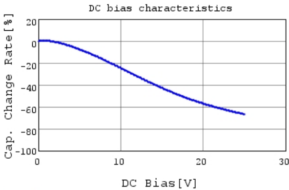
GCM21BR71E225KA73 C-DC bias capchange, 25.0c
