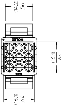
PLUG 1292-P1 SHOWN
