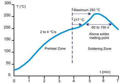
Fig. 2. Reflow Temperature Profile for Pb-free Soldering
