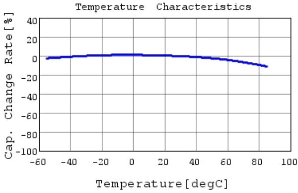
GRM155R61A105KE15 C-Temp. capchange, DC0.0V,
