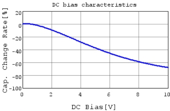
GRM155R61A105KE15 C-DC bias capchange, 25.0c
