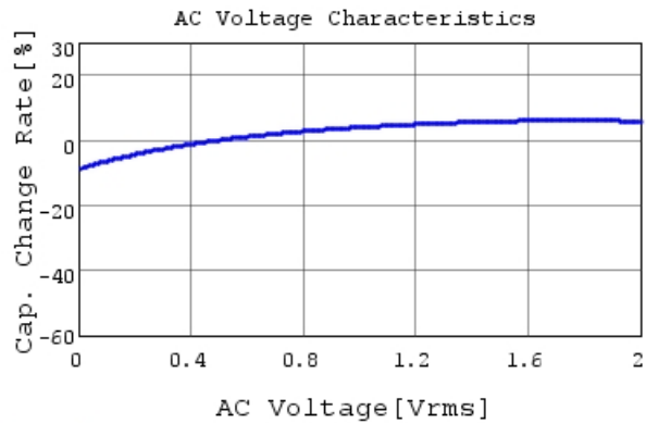
GRM155R61A105KE15 C-AC Voltage capchange, Dc
