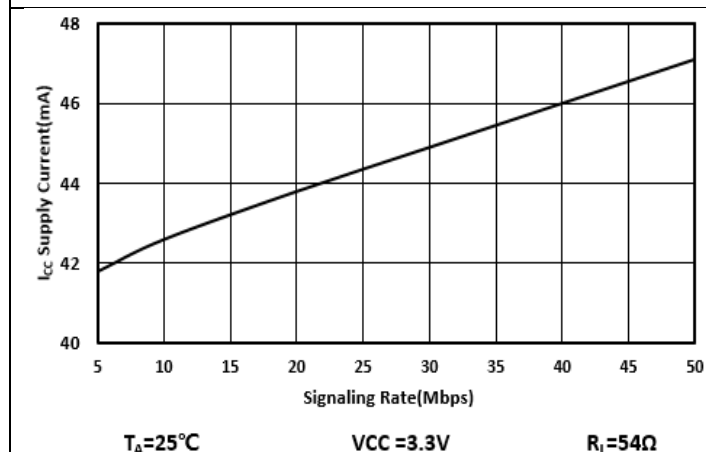
图 20 I_{CC} Supply Current vs Signaling Rate
