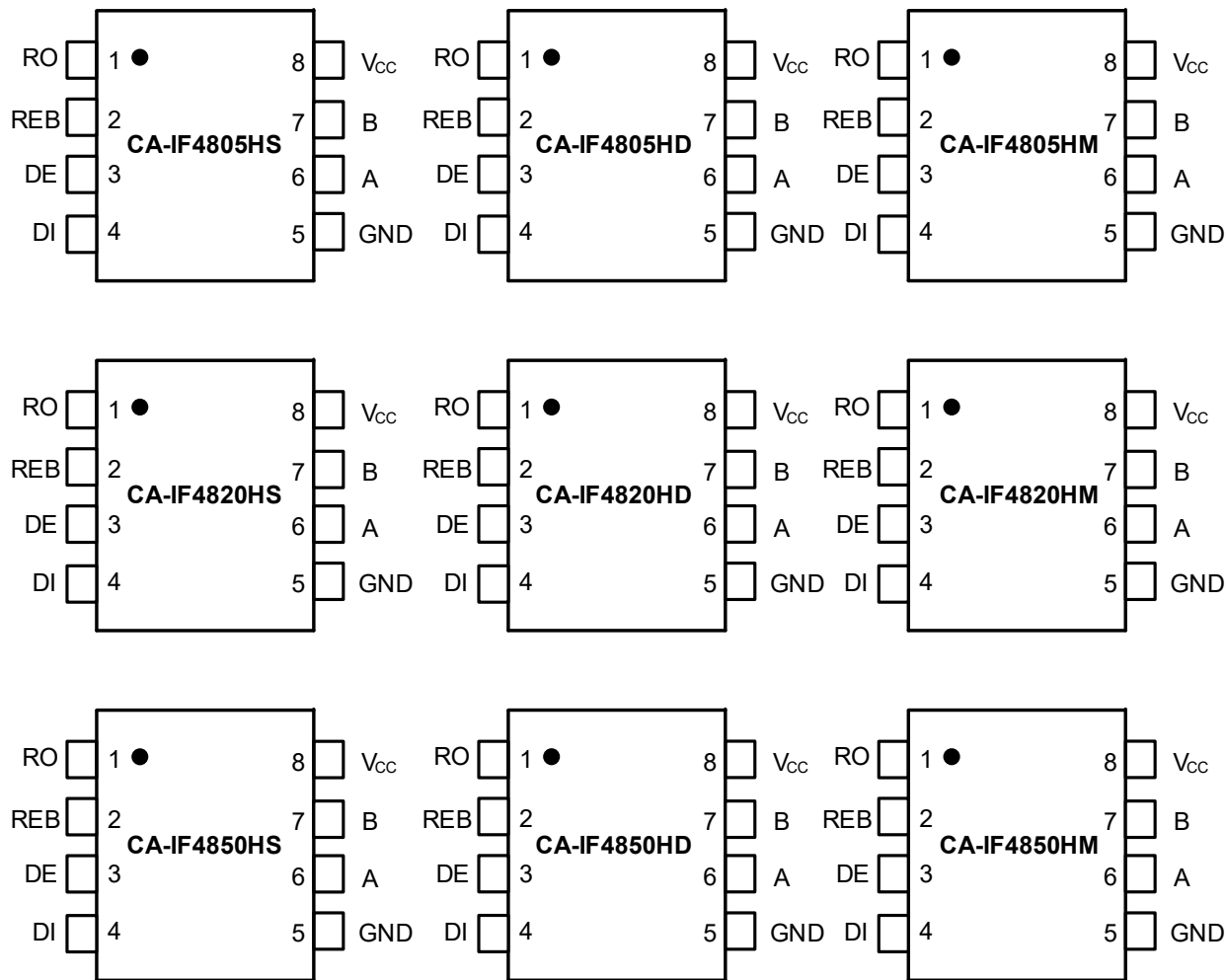
图 1 CA-IF48xxHS/CA-IF48xxHD/CA-IF48xxHM 引脚图
