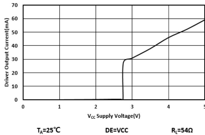
图 11 Driver Output Current vs Supply Voltage
