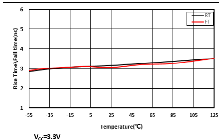
图 18 Rise Time\Fall Time vs Temperature
