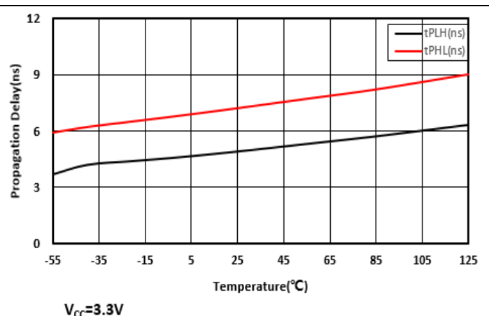
图 19 Propagation Delay vs Temperature
