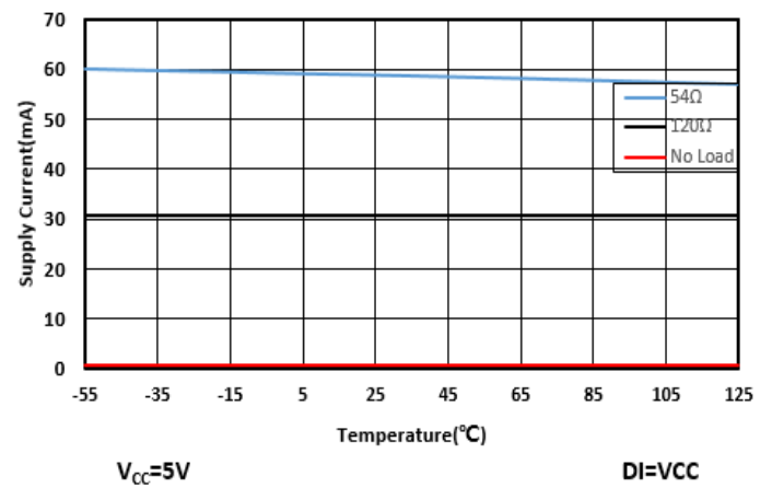
图 10 Quiescent Current vs Temperature
