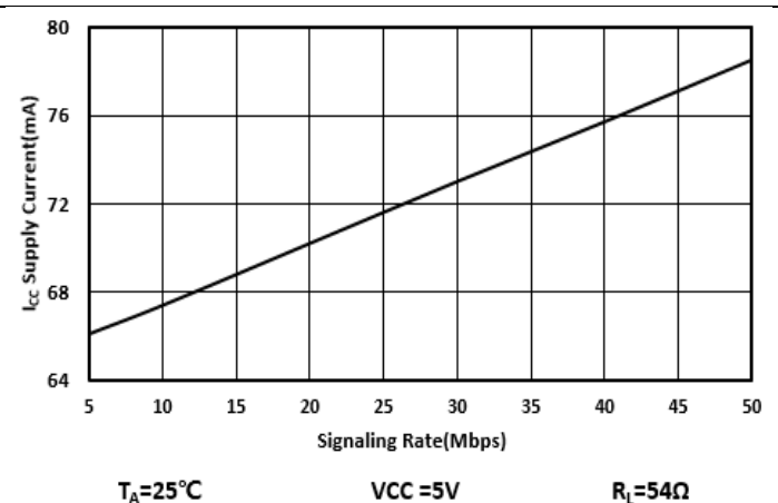
图 23 I_{CC} Supply Current vs Signaling Rate
