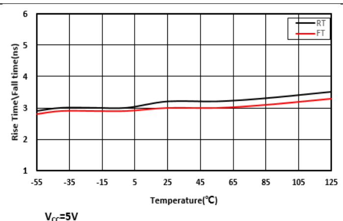
图 21 Rise Time\Fall Time vs Temperature
