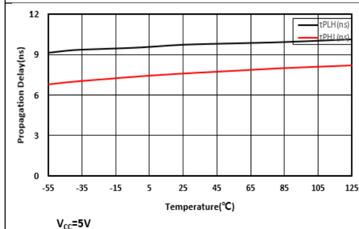
图 22 Propagation Delay vs Temperature
