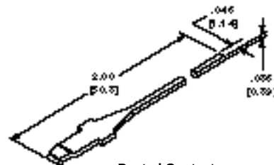
Posted Contact
