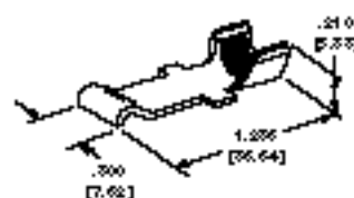
Solder Contact
