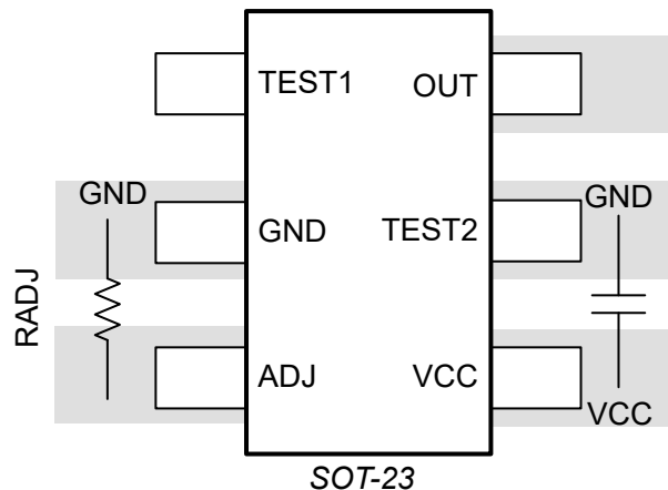
Figure 10-1. Layout Examples
