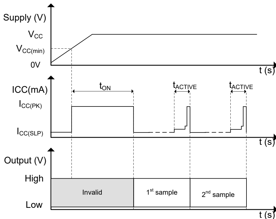
Figure 7-4. Timing Diagram
