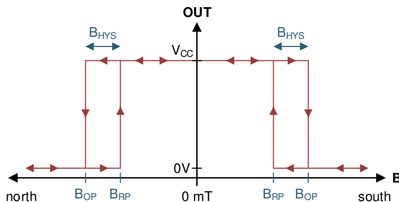
Figure 7-2. Omnipolar Functionality
