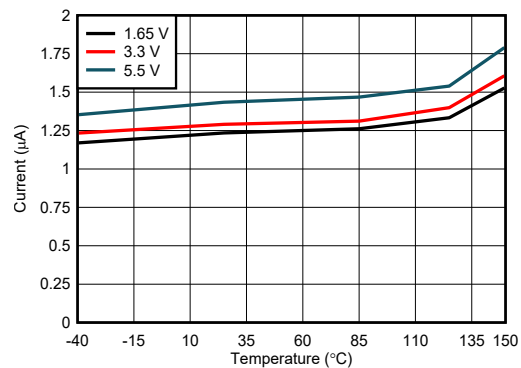
Figure 6-7. Average I_{CC} vs Temperature
