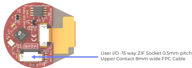
FPC Pinout
