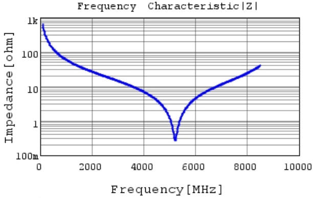
GJM1555C1H2R6BB01 |Z| DCOV, 25degC
