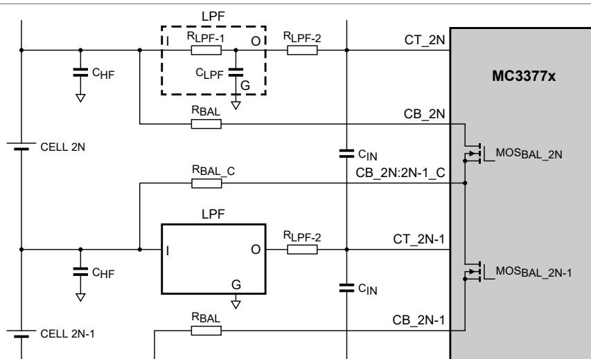
Figure 39. LPF block masking
