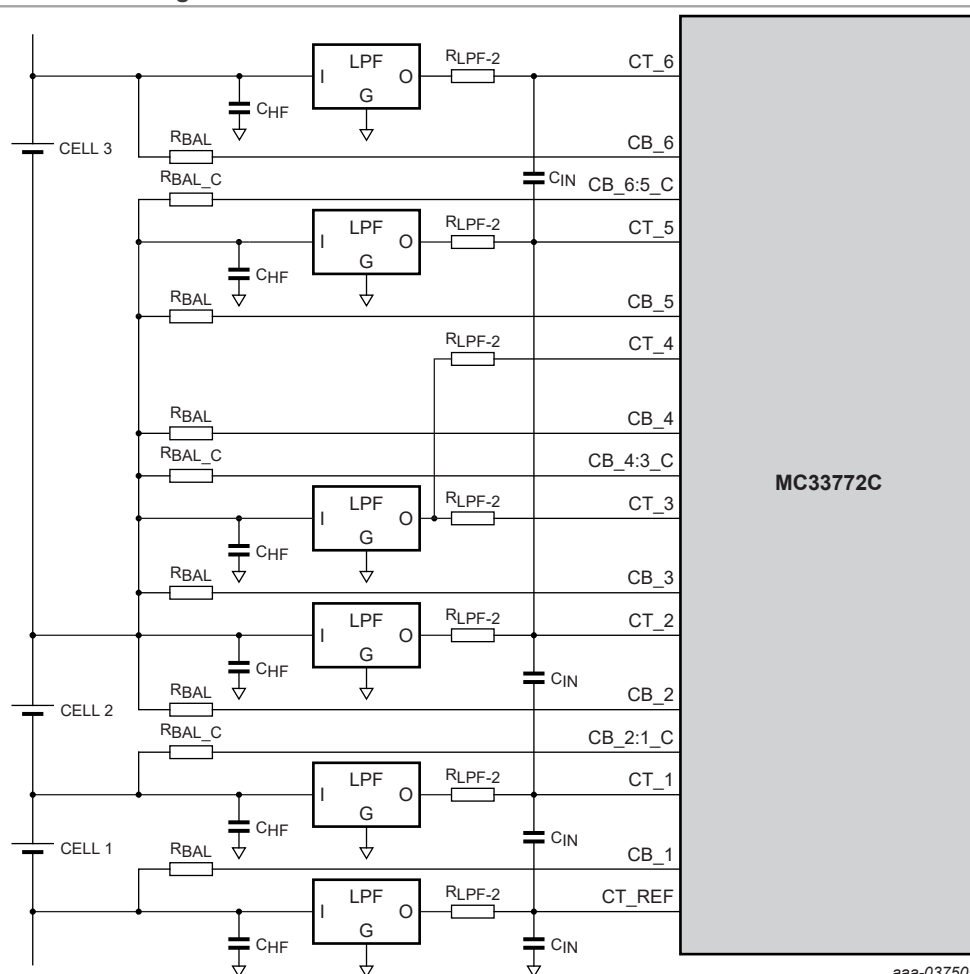
Figure 40. The three cell configuration
