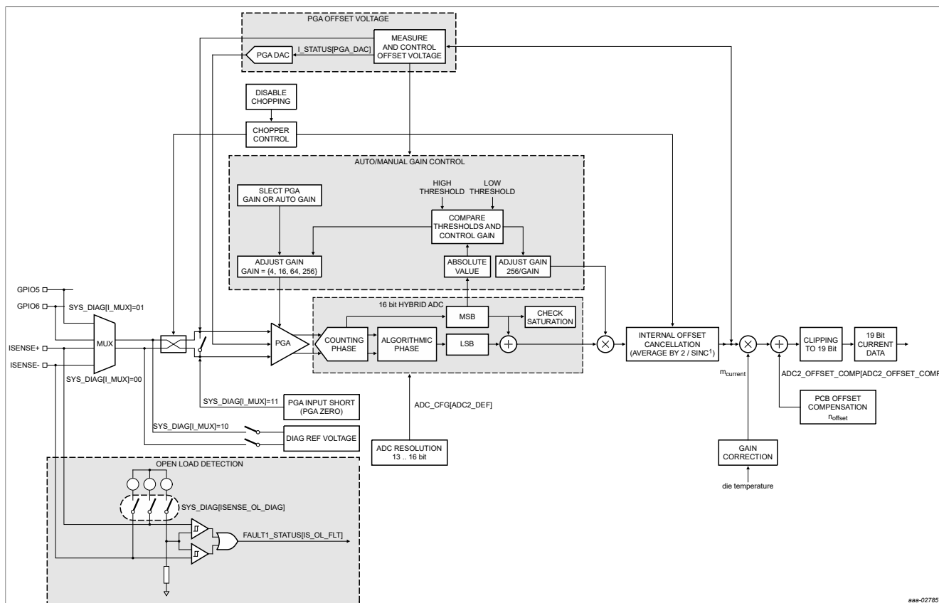
Figure 12. Current measurement channel
