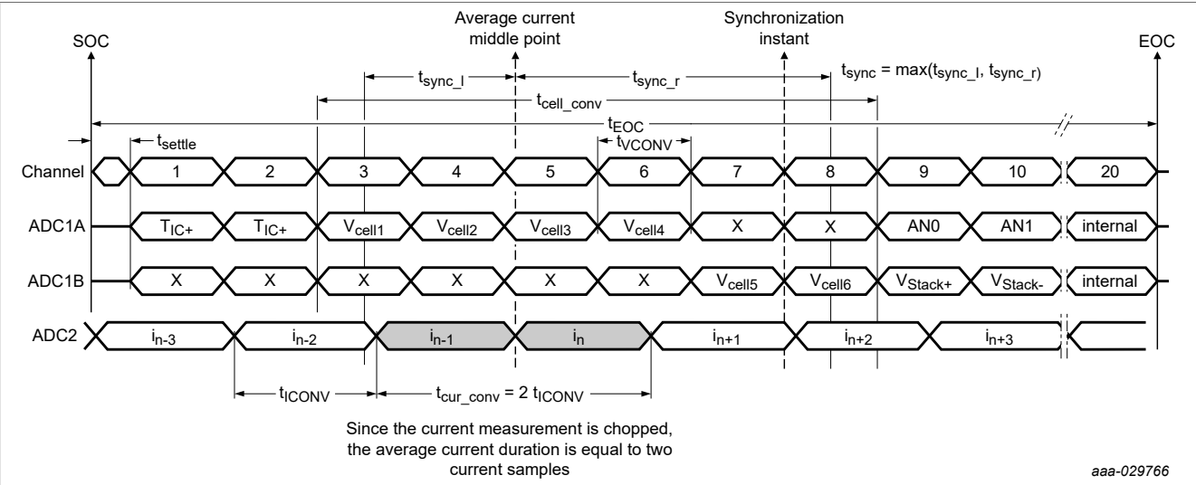
Figure 10. ADC conversion sequence in normal mode
