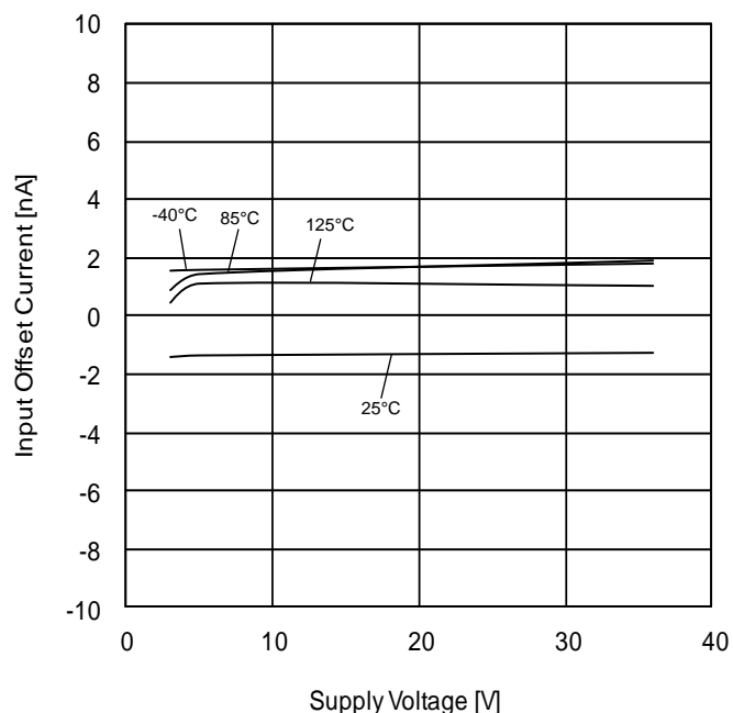
Figure 48. Input Offset Current vs Supply Voltage ( V_{ICM}=V_{CC}/2 , E_K=-V_{CC}/2 )
