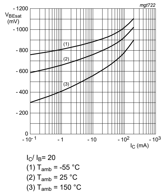
Fig. 15. BC857CQB-Q: Base-emitter saturation voltage as a function of collector current; typical values
