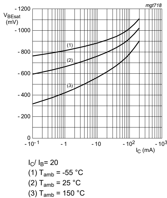
Fig. 11. BC857BQB-Q: Base-emitter saturation voltage as a function of collector current; typical values
