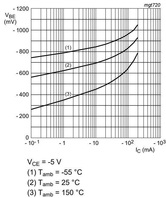
Fig. 13. BC857CQB-Q: Base-emitter voltage as a function of collector current; typical values
