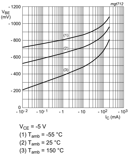
Fig. 5. BC857AQB-Q: Base-emitter voltage as a function of collector current; typical values
