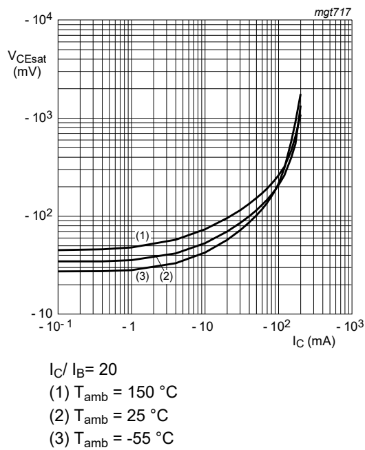
Fig. 10. BC857BQB-Q: Collector-emitter saturation voltage as a function of collector current; typical values
