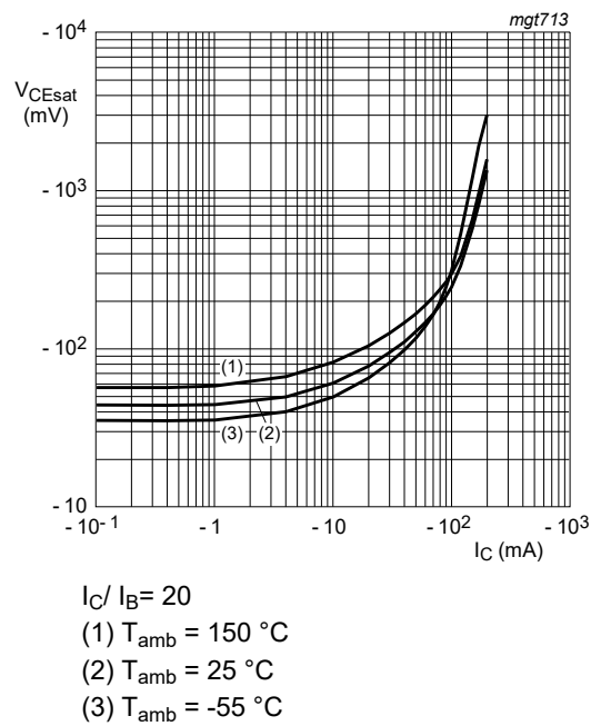
Fig. 6. BC857AQB-Q: Collector-emitter saturation voltage as a function of collector current; typical values
