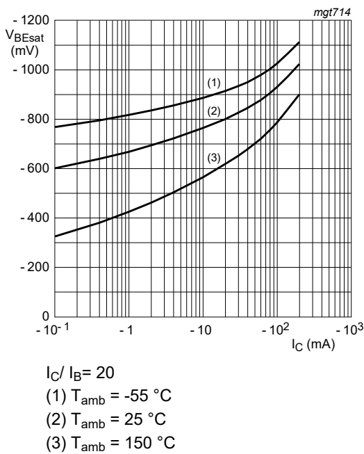
Fig. 7. BC857AQB-Q: Base-emitter saturation voltage as a function of collector current; typical values
