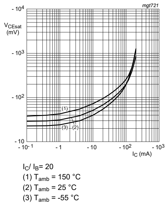
Fig. 14. BC857CQB-Q: Collector-emitter saturation voltage as a function of collector current; typical values
