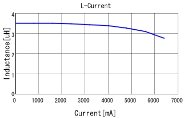
B1047AS-3R6N L-Current 20degC
