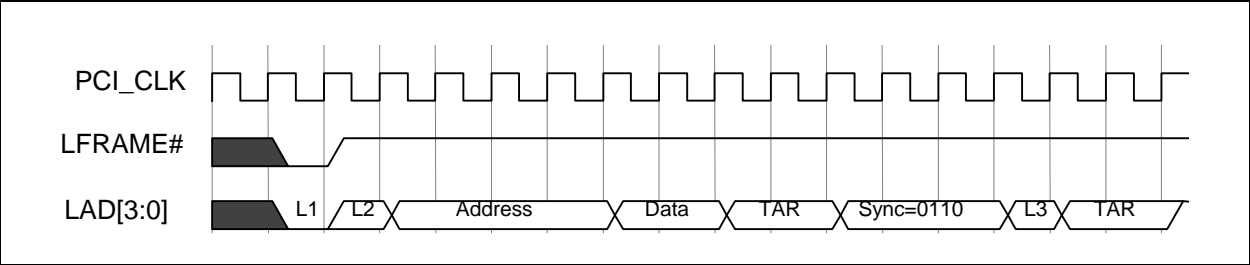
FIGURE 29-7: I/O WRITE
