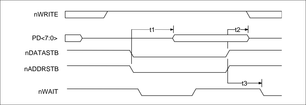
FIGURE 29-16: EPP 1.7 DATA OR ADDRESS READ CYCLE
