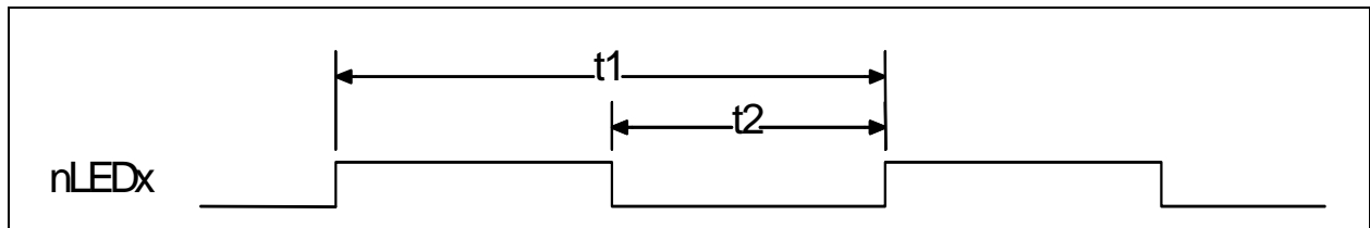
FIGURE 29-30: NLEDX TIMING
