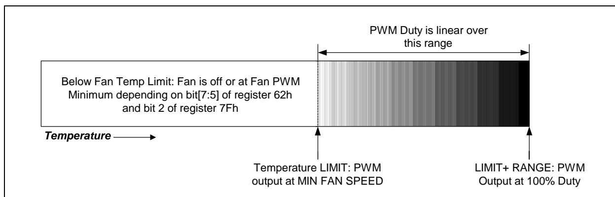
FIGURE 24-1: FAN ACTIVITY ABOVE FAN TEMP LIMIT
