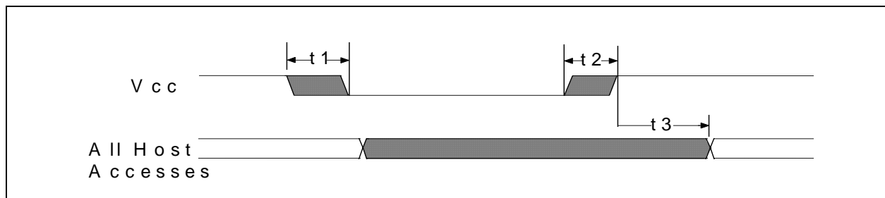
FIGURE 29-1: POWER-UP TIMING
