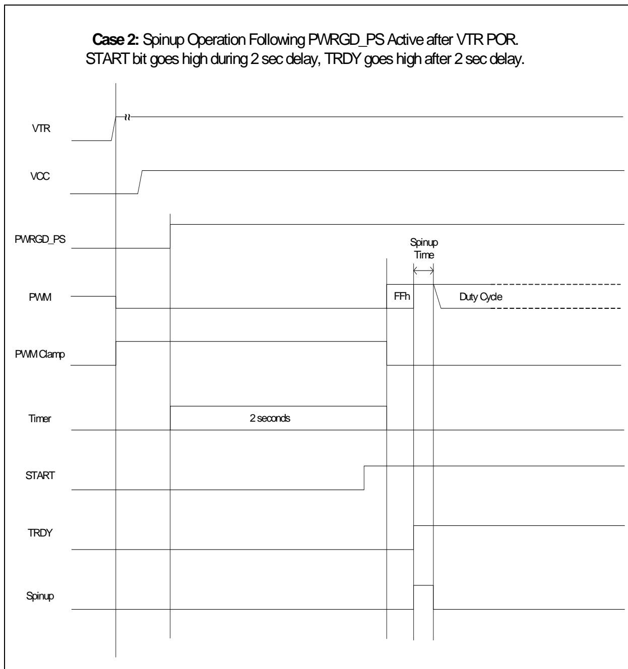
FIGURE 23-9: CASE 2 SPINUP OPERATION
