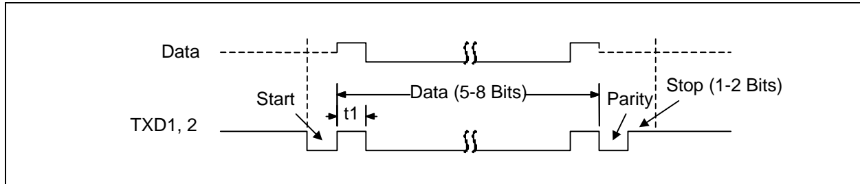
FIGURE 29-25: SERIAL PORT DATA
