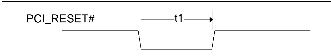
FIGURE 29-4: RESET TIMING
