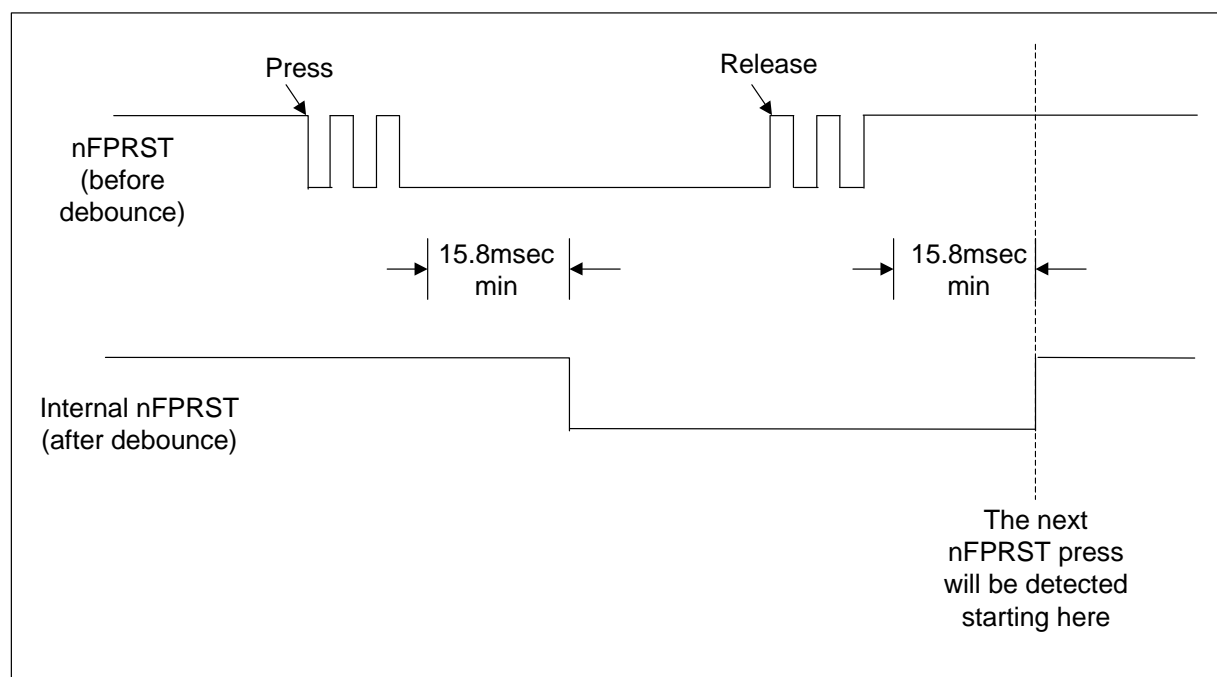
FIGURE 20-2: NFPST DEBOUNCE TIMING
