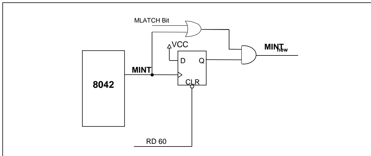
FIGURE 12-4: MOUSE LATCH
