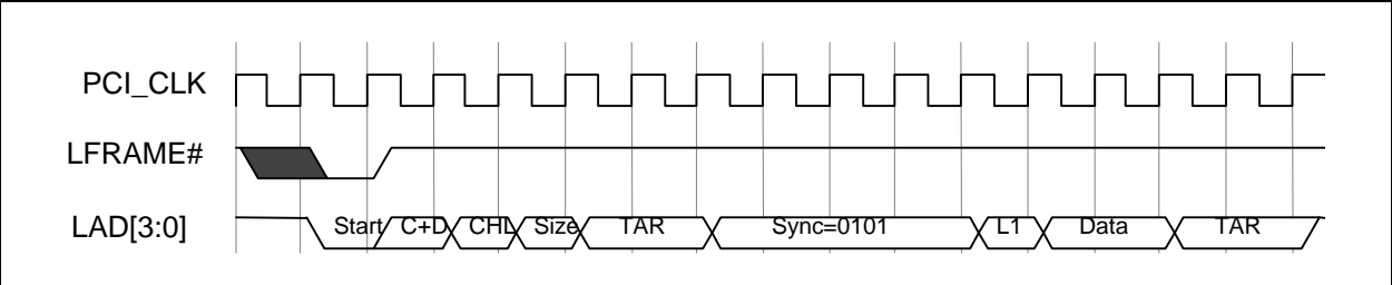
FIGURE 29-10: DMA WRITE (FIRST BYTE)
