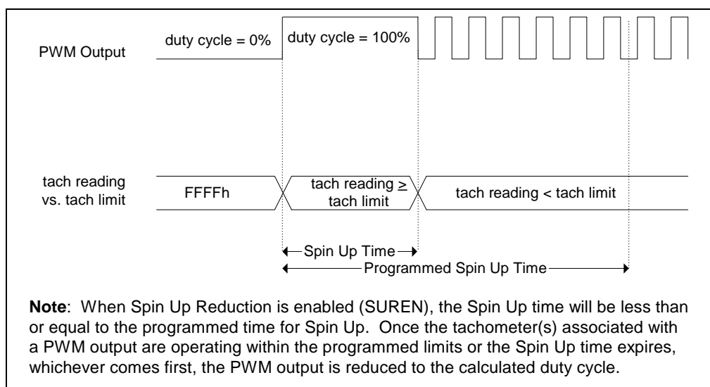
FIGURE 23-6: SPIN UP REDUCTION ENABLED
