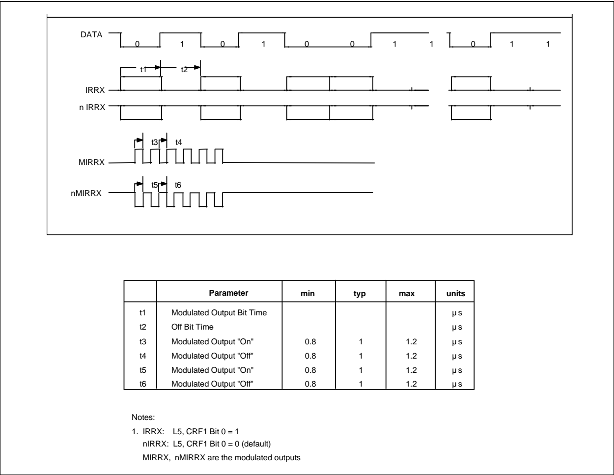
FIGURE 29-22: AMPLITUDE SHIFT-KEYED IR RECEIVE TIMING
