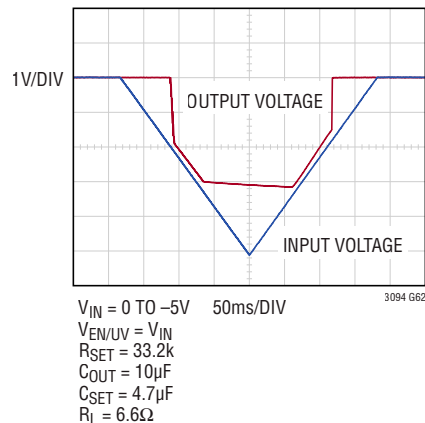
Input Supply Ramp-Up and Ramp-Down
