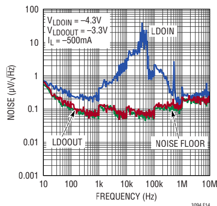
Figure 14. LT3094's Input and Output Noise Spectral Density
