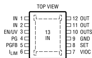
MSE PACKAGE 12-LEAD PLASTIC MSOP T_{JMAX} = 150^{\circ}\text{C} , \theta_{JA} = 33^{\circ}\text{C/W} , \theta_{JC} = 8^{\circ}\text{C/W} EXPOSED PAD (PIN 13) IS IN, MUST BE SOLDERED TO PCB
