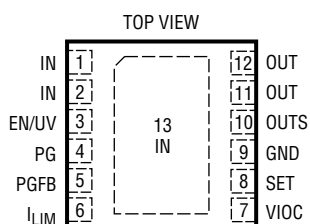
DD PACKAGE 12-LEAD (3mm × 3mm) PLASTIC DFN T_{JMAX} = 150^{\circ}\text{C} , \theta_{JA} = 34^{\circ}\text{C/W} , \theta_{JC} = 5.5^{\circ}\text{C/W} EXPOSED PAD (PIN 13) IS IN, MUST BE SOLDERED TO PCB
