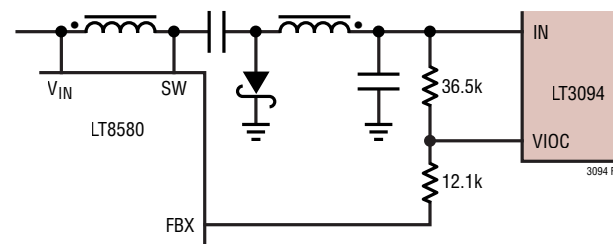
Figure 9. VIOC Connection Using LT8580
