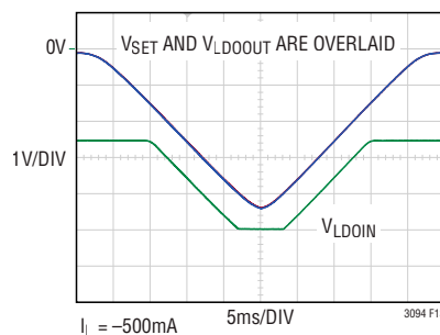
Figure 13. Ramping V SET from 0V to -4.5V (and Back to 0V)
