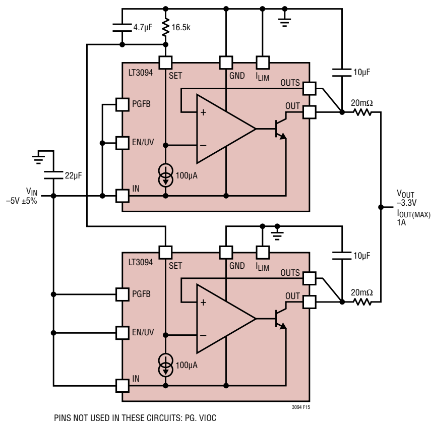
Figure 15. Parallel Devices
