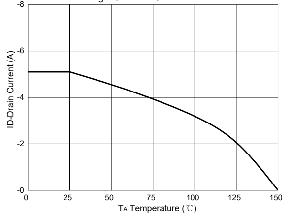
Fig. 10 - Drain Current
