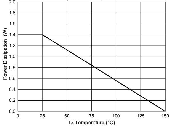
Fig.11-PD Dissipation
