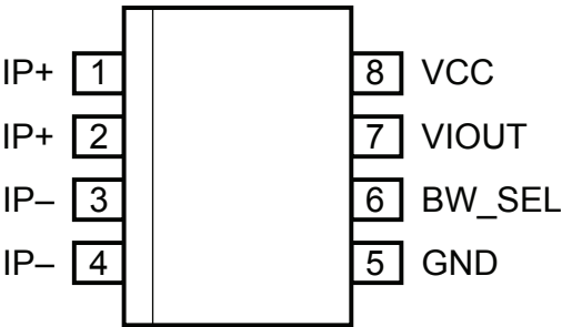
Pinout Diagram
