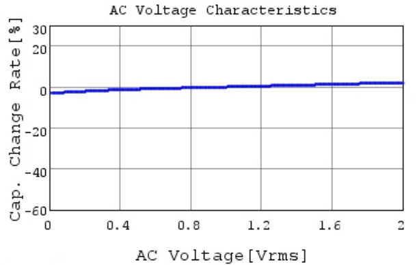
GRM155R72A472KA01 C-AC Voltage capchange, Dc
