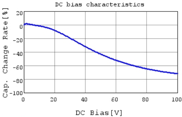
GRM155R72A472KA01 C-DC bias capchange, 25.0c
