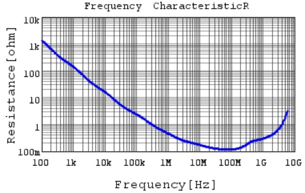
GRM155R72A472KA01 R DCOV, 25degC
