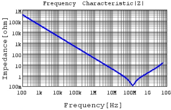
GRM155R72A472KA01 |Z| DCOV, 25degC
