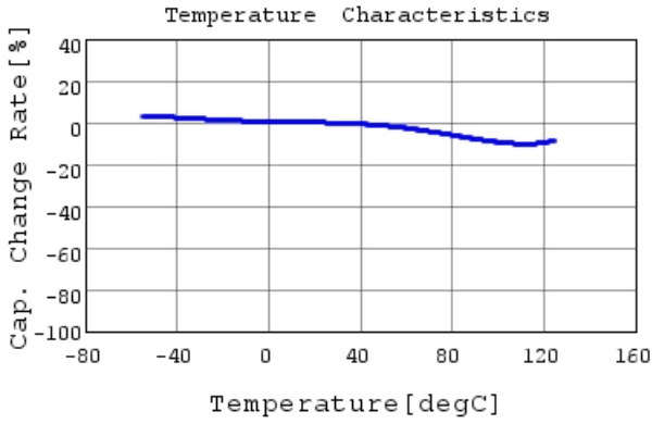
GRM155R72A472KA01 C-Temp. capchange, DC0.0V,
