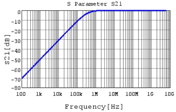
GRM155R72A472KA01 S21 DC0V, 25degC
