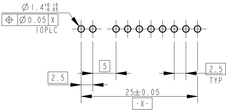
3 REFERENCE PCB LAYOUT FOR 1717445-1
