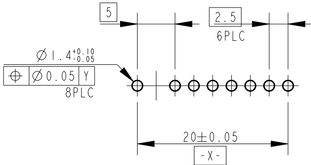
3 REFERENCE PCB LAYOUT FOR 1717445-4/-5/-6
