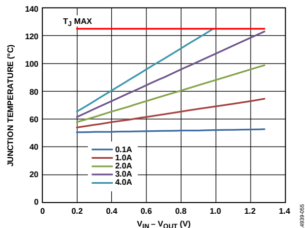
Figure 55. 100 mm 2 of PCB Copper, T_B = 50^\circ\text{C} , LFCSP
