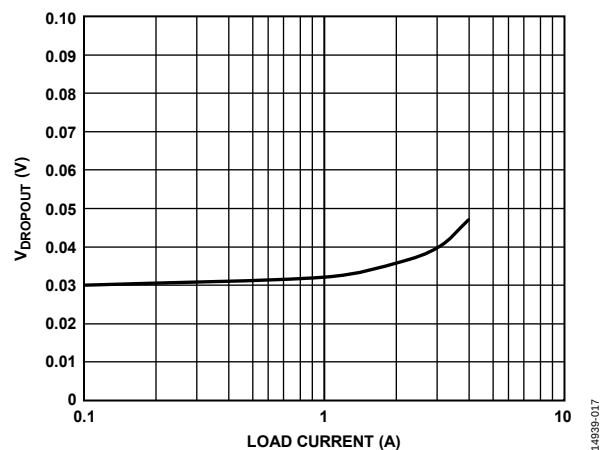
Figure 17. Dropout Voltage ( V_{DROP} ) vs. Load Current ( I_{LOAD} ), V_{OUT} = 1.3V
