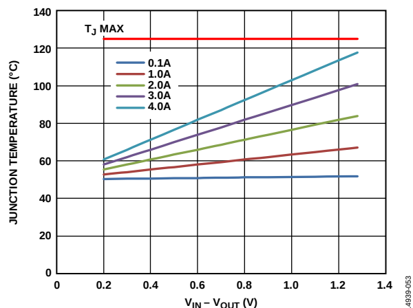
Figure 53. 1000 mm 2 of PCB Copper, T_B = 50^\circ\text{C} , LFCSP
