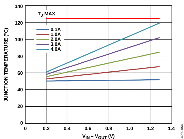
Figure 54. 500 mm 2 of PCB Copper, T_B = 50^\circ\text{C} , LFCSP
