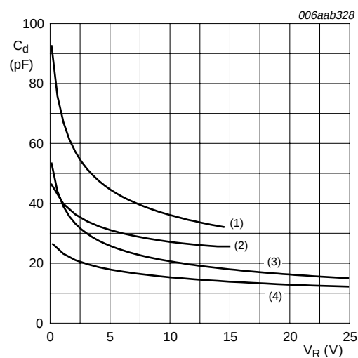
f = 1 \text{ MHz}; T_{\text{amb}} = 25^\circ\text{C} (1) MMBZ15VDL: unidirectional (2) MMBZ15VDL: bidirectional (3) MMBZ27VCL: unidirectional (4) MMBZ27VCL: bidirectional
