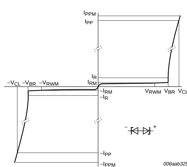
Fig 8. V-I characteristics for a bidirectional ESD protection diode
