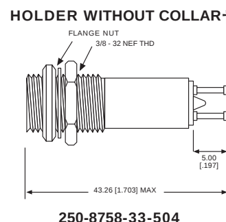
HOLDER WITHOUT COLLAR†
