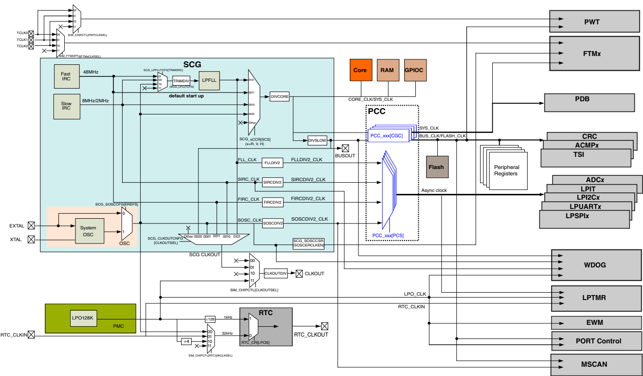
Figure 3. Clocking block diagram
