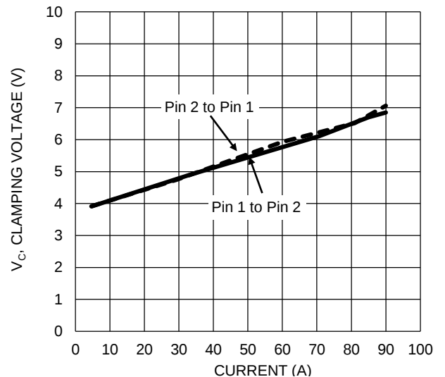
Figure 6 Clamping Voltage Characteristic ( t_p = 8/20\mu s )
