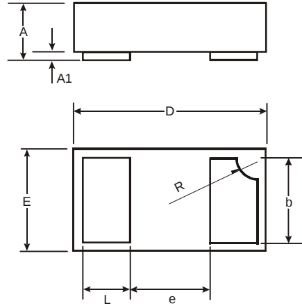
X1-DFN1006-2
