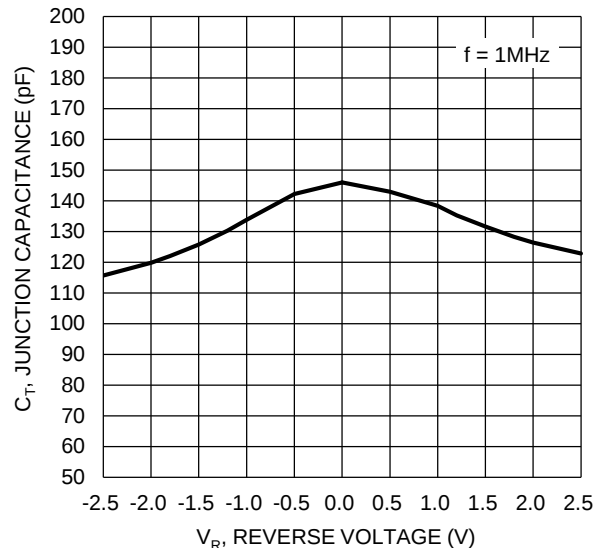
Figure 4 Typical Pin1 to Pin2 Capacitance
