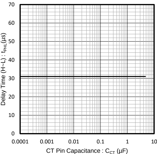
Figure 28. Output Delay Time (H to L)
