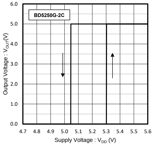
Figure 15. Detection Voltage
