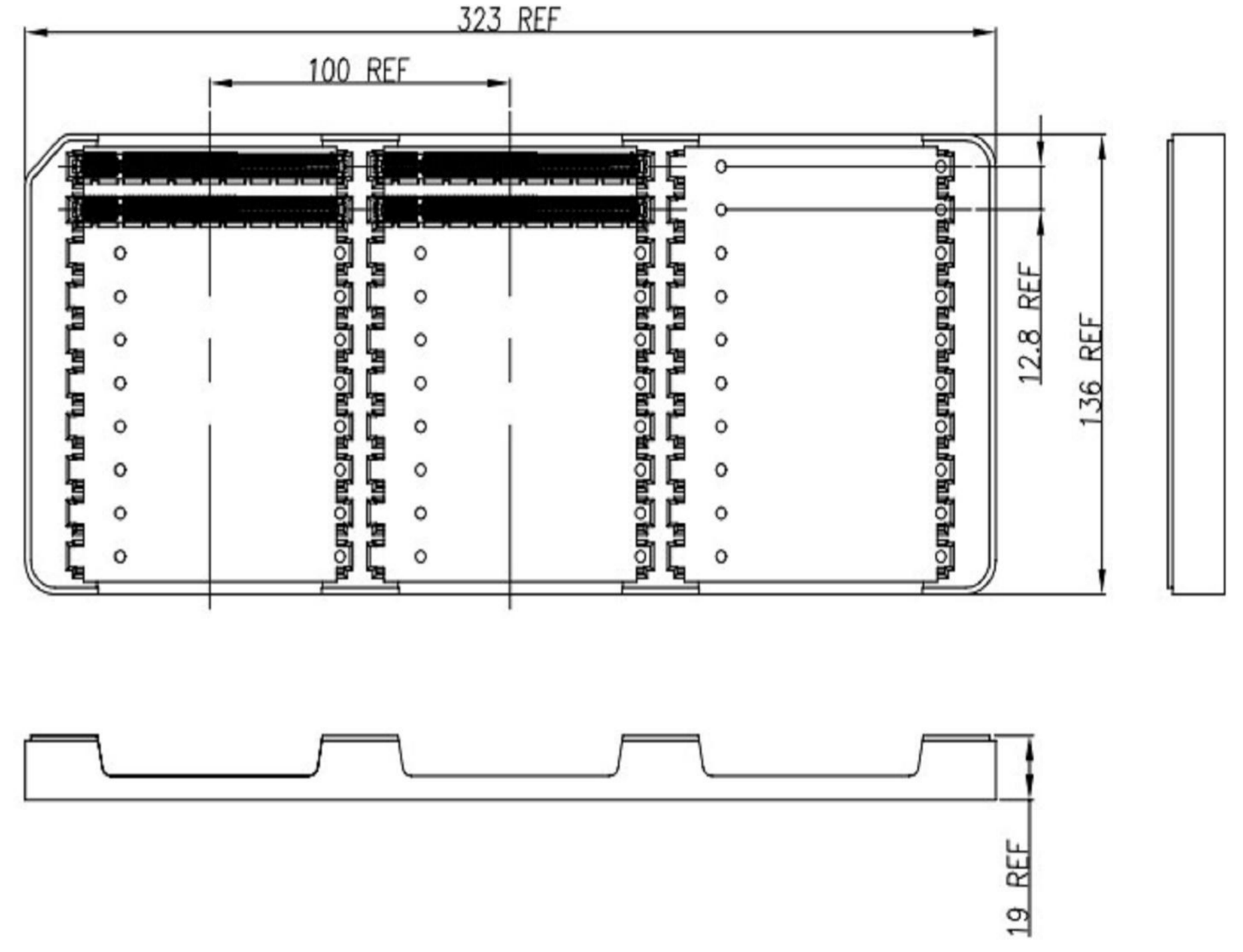
HARD TRAY: FOR 6-2364427-7/8/9 (164POS) SCALE: 1:2
