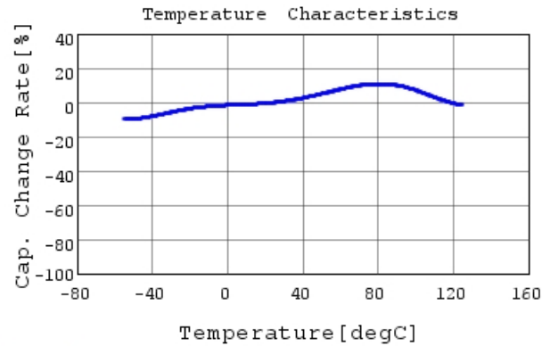
GRM155R71A474KE01 C-Temp. capchange, DC0.0V,
